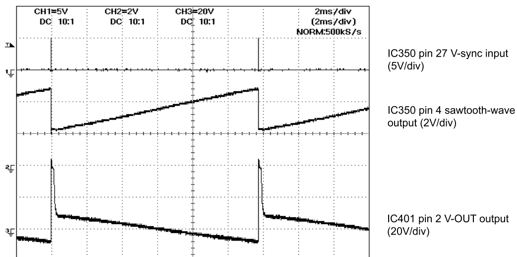
<Vertical Waveform>
